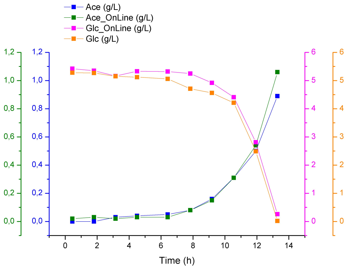
Figure 1. Online HPLC measurements compared to stand-alone HPLC.
